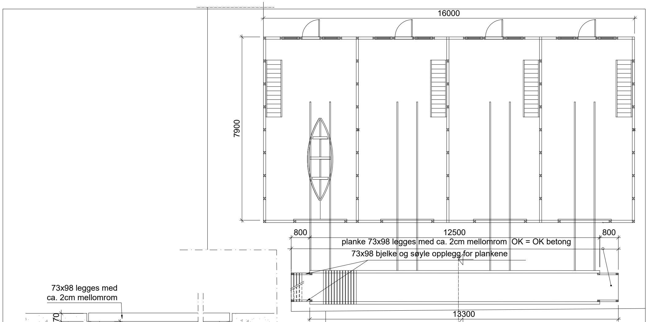
Plantegning naust, 1:100
