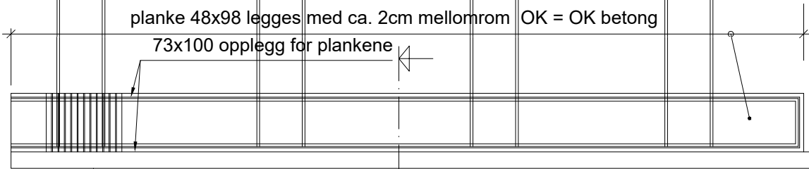
Plantegning naust, 1:100
